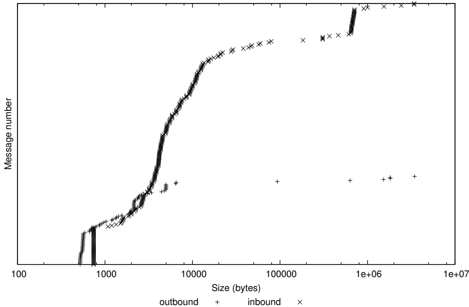
Email Message Sizes
